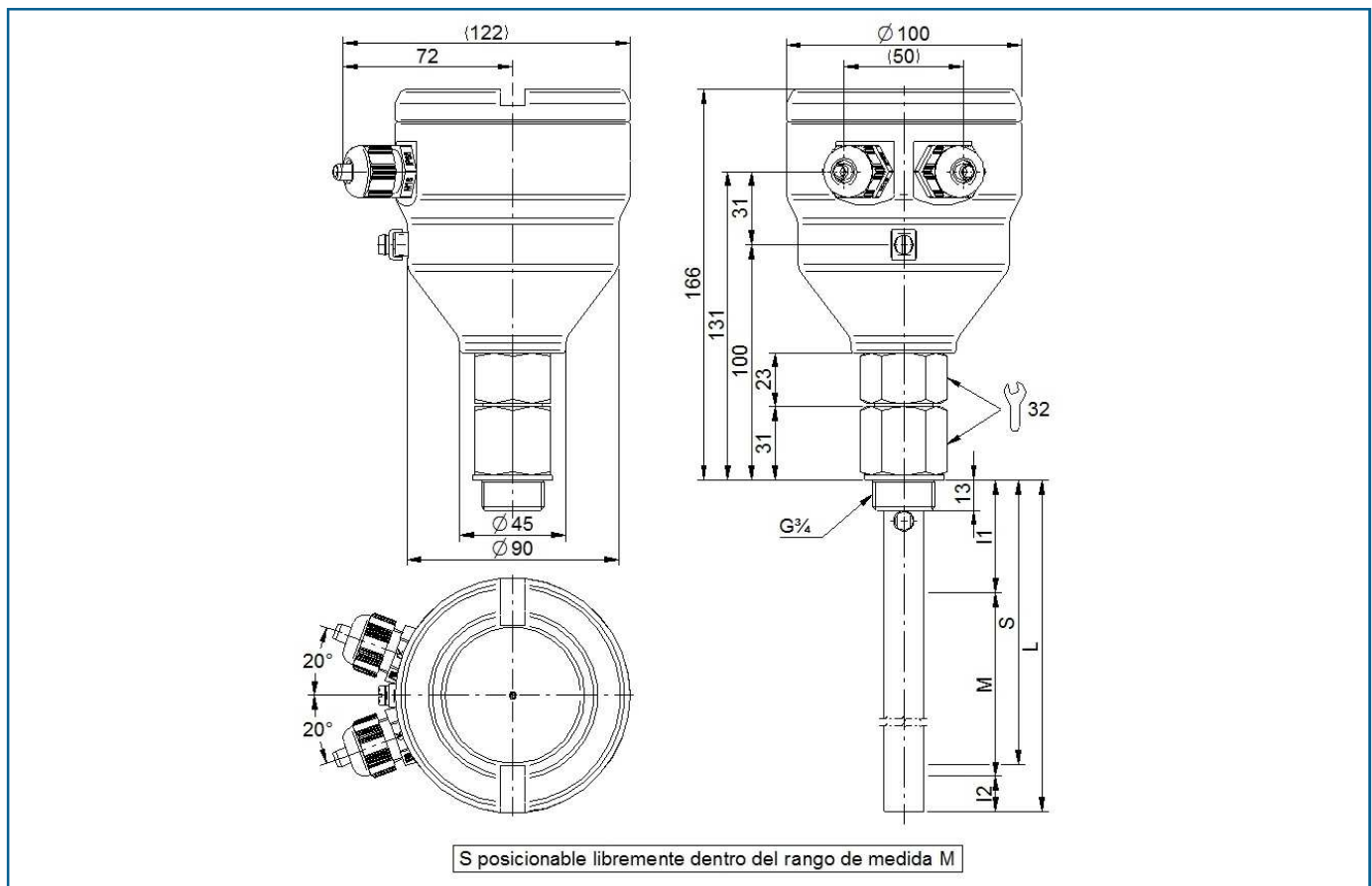
Fig. 4. Sonda coaxial
